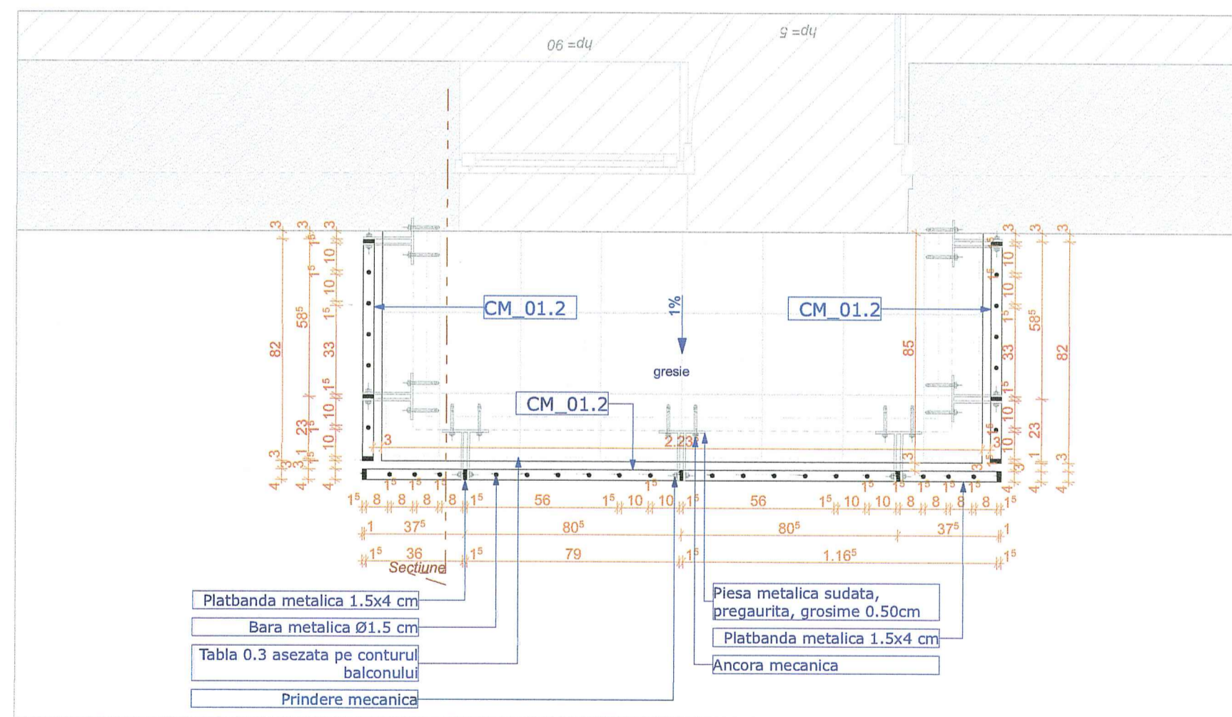
Plan CM_01 SC 1:20
